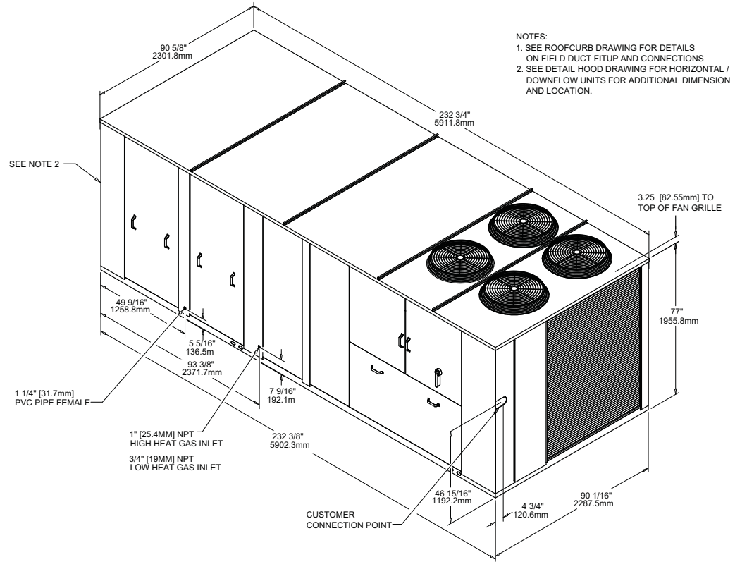
Figure 21. 60 Hz 40-50, 50 Hz 33-42 tons (TC, TE, YC low and high heat)
