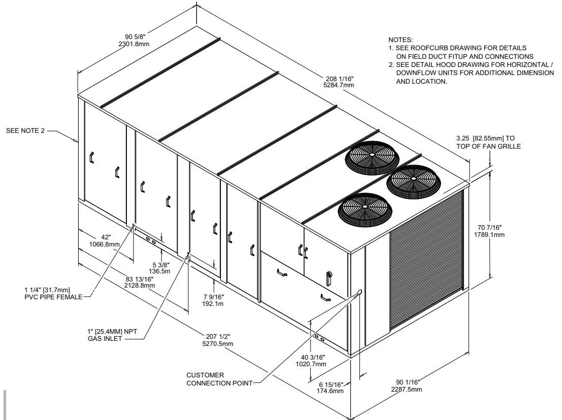
Figure 17. 60 Hz 27½-35, 50 Hz 23-29 tons (YC high heat)
