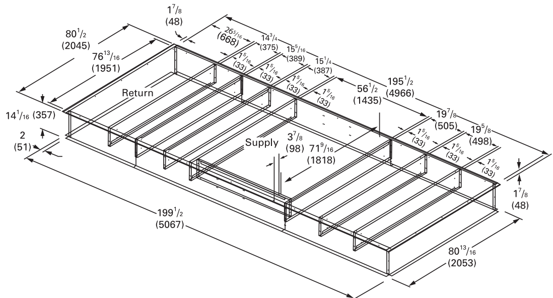
Figure 18. Curb assembly, 60 Hz 27½-35, 50 Hz 23-29 tons (YC high heat)
