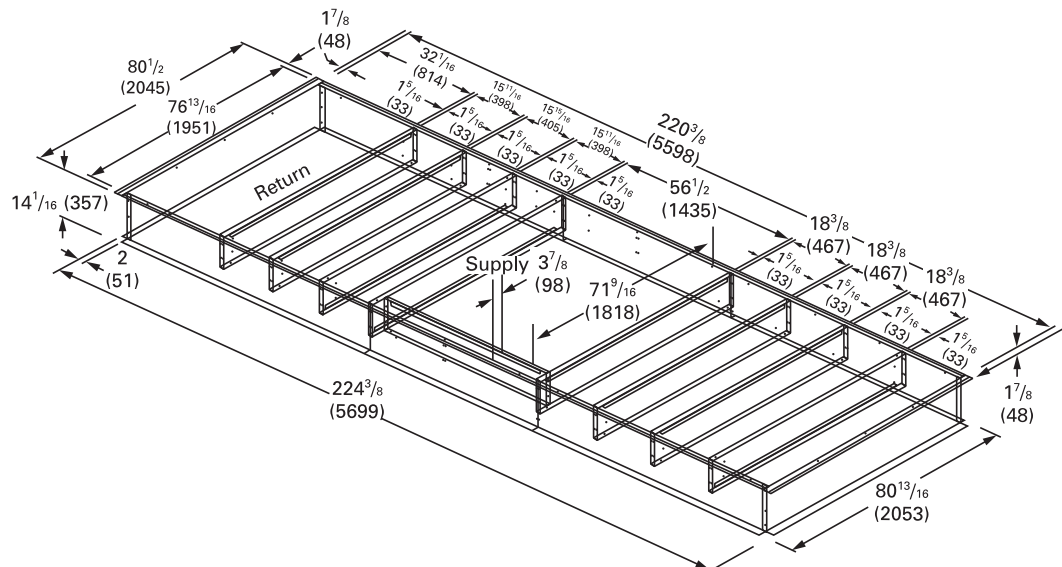
Figure 22. Curb assembly, 60 Hz 40-50, 50 Hz 33-42 tons (TC, TE, YC low and high heat)
